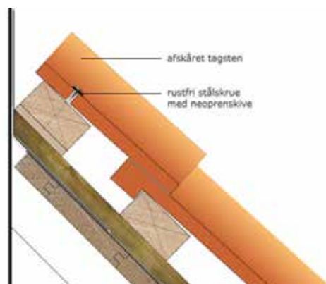
Skruemontering
